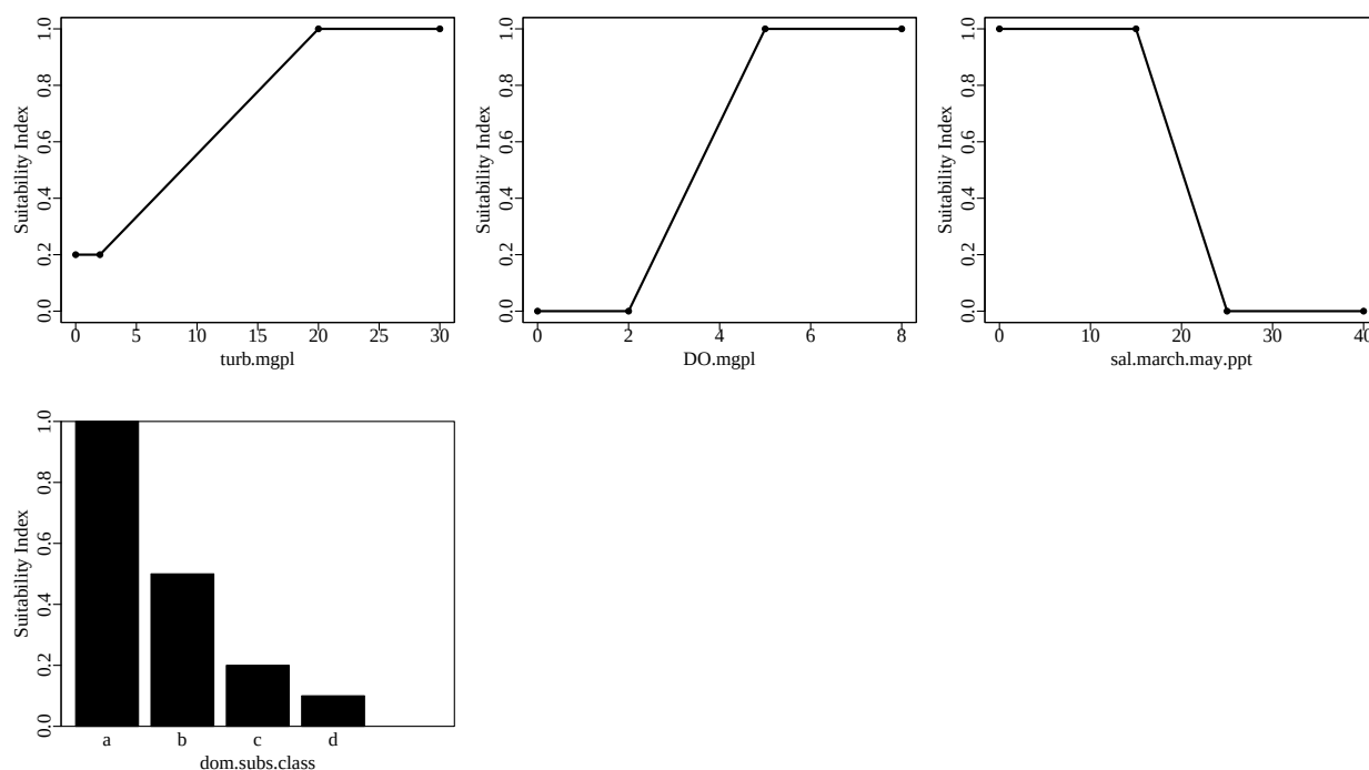
Figure 1. Suitability index graphs for variables included in the atlanticcroakerLATideMt0.5m model in ecorest.
